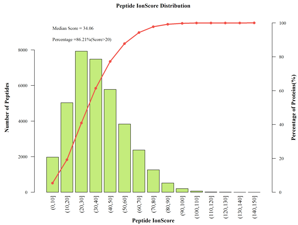
Supplementary Fig. 4 Tool of MASCOT in judging each MS2 spectrograms, the median score is 34.06, and more than 86.21% peptides are score higher than 20. Red line means the cumulative curve.
