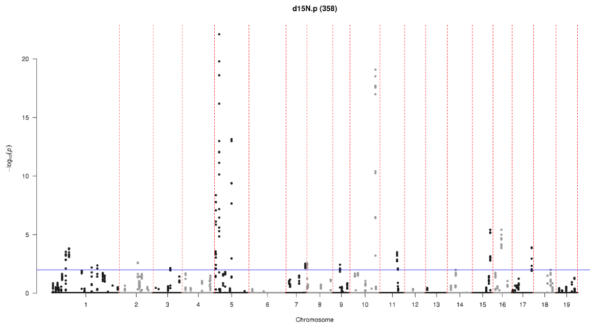
Figure S3. Manhattan plots for sliding window analysis tests.
