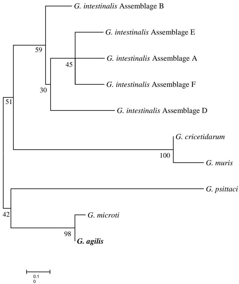
Phylogenetic tree from ML based on \beta -giardin sequences indicating that G. agilis is distinct from all Giardia spp.
